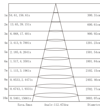
Illuminance-Distance Curve
