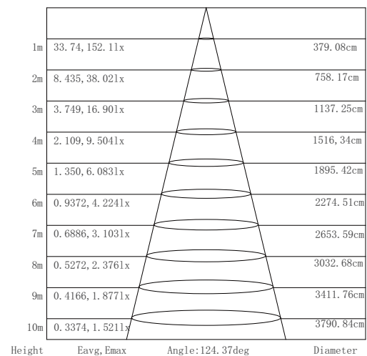
Illuminance-Distance Curve
